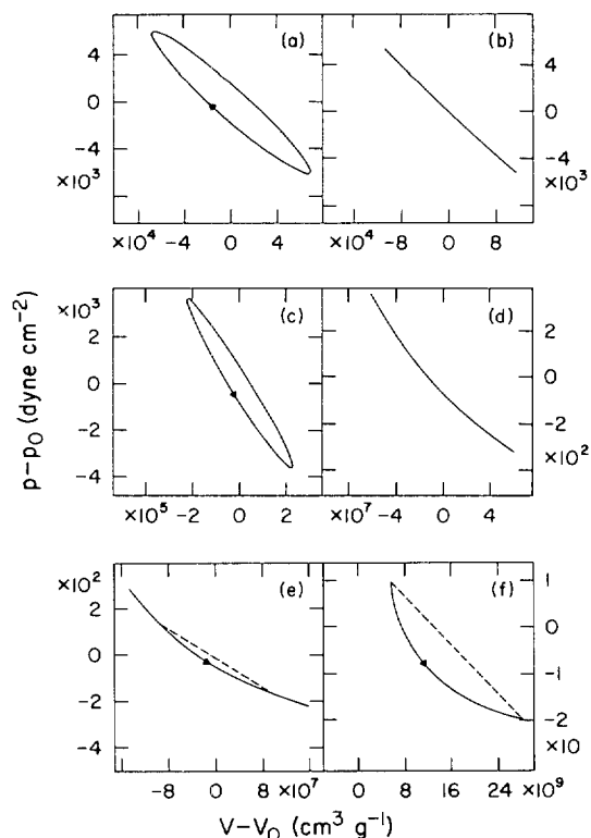
Fig. 105.5 Thermodynamic cycles in (p, V) plane. Initial heights: (a) -44 \text{ km} , (b) 11 \text{ km} , (c) 88 \text{ km} , (d) 550 \text{ km} , (e) 616 \text{ km} , (f) 946 \text{ km} . From (U6), by permission.
